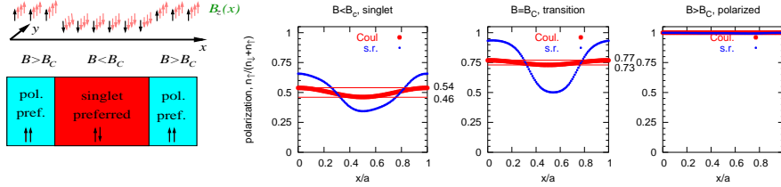
Fig. 2. Response of the ground state (singlet, at the transition and polarized) for H_{\text{Coul}} and H_{\text{hc}} to magnetic inhomogeneity of the profile shown on the left (supporting domain formation: domain structure expected for uncorrelated electrons shown on left). For Coulomb-interacting system monotonous transition is observed (polarization variation at B = B_C is half the variation for the singlet GS); the transition state (at B = B_C ) in short-range-interacting systems might form domains. Strength of the MI is 6% and 25% of the singlet GS gap for the Coulomb and short-range interaction, respectively.
